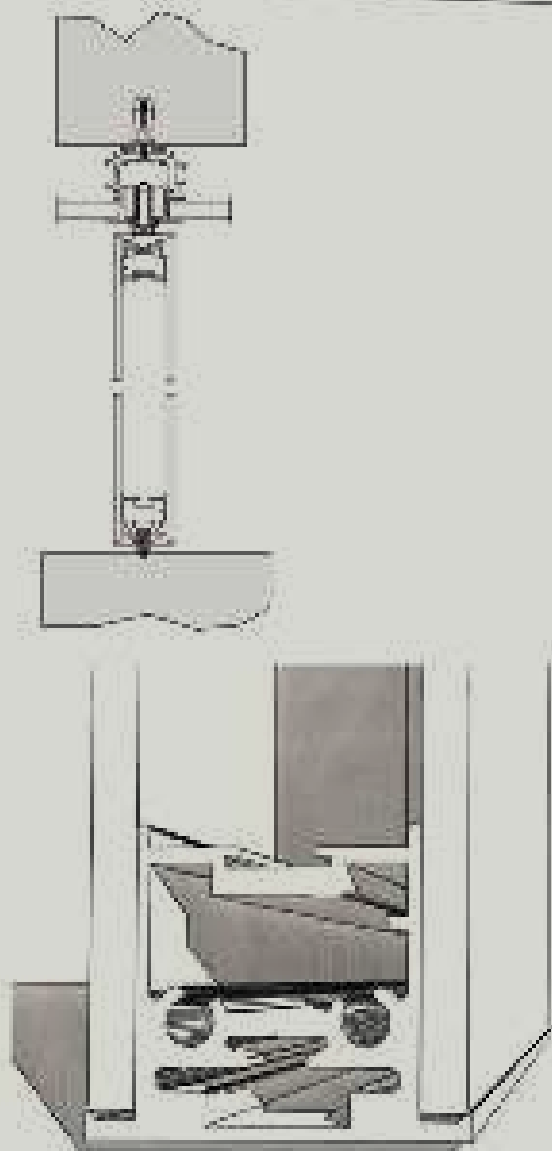
Ceiling sliding system for plasterboard. Single or double door panels with perimetrical aluminum profile and double glass.
